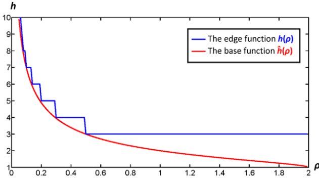
Figure 5: A graph of the edge number function h(\rho) (blue) and its continuous basis function \hat{h}(\rho) (red), where the variable of two functions is \rho , the error on internode polygonization.
