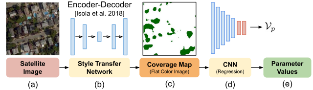
Fig. 13. Neural network pipeline: we use a style-transfer network (b) trained on data pairs from NYCOpenData [2019] to convert satellite images (a) to coverage maps (c). To learn parameter values for our PPMs (for which no ground truth data for satellite images exist) we generate pairs of coverage maps and parameter values with the PPMs of our framework. We then train a CNN (d) to obtain parameter values (e) for the estimated coverage maps of the real satellite images.
