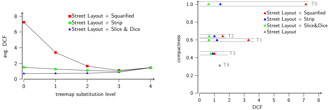
Figure 5: Stability (on the left) and compactness (both together on the right) analysis of Street Layout in combination with different Treemap approaches based on 5x4 hierarchies. The substitution level indicates the level in the hierarchy from which the elements are represented through Treemaps. Level 0 corresponds to a complete Treemap and level 4 to an unmodified Street Layout.
