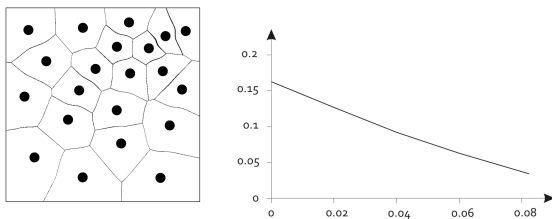
Figure 8: Voronoi Diagram of a set of disks and values of F_{min} for different disk radii.
