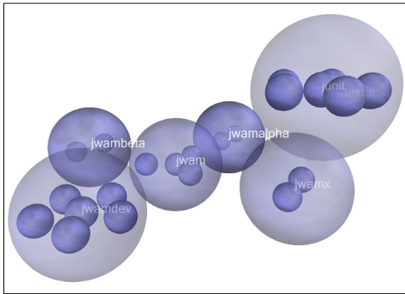
Figure 2: Representation of the package hierarchy of the software system 'JWAM 1.6' using nested spheres
