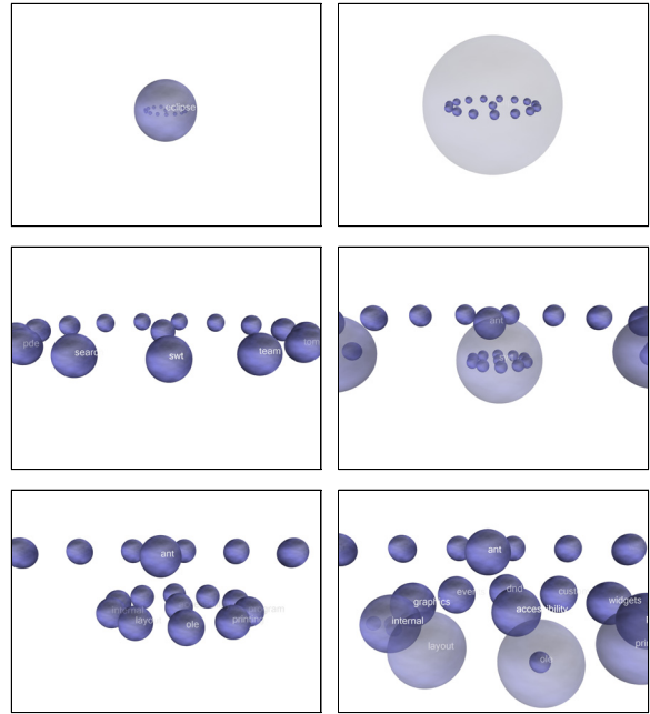
Figure 3: Changing sphere transparencies when zooming into the package hierarchy of the software system 'Eclipse 2.02'; Far upper left: Overview of the entire software system; Far lower right: Closeup view of selected packages of the software system
