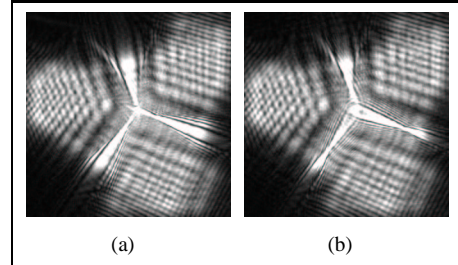
Figure 12: A simple coordinate system, reconstructions at distinct depths
