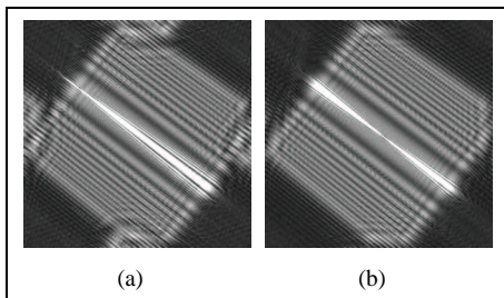
Figure 11: Two simulated reconstructions of a line segment at a (a) nearer and (b) bigger distance from the hologram
